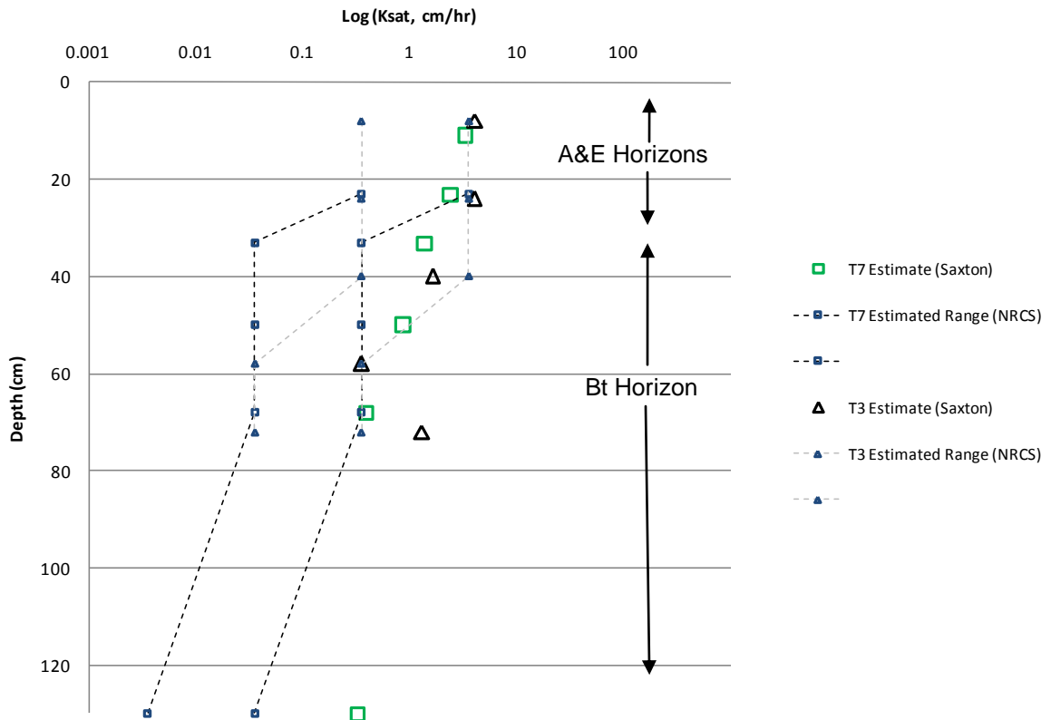
Figure 15. UF Upland Landscape Unit: Direct Measurements and Indirect Estimates of Saturated Hydraulic Conductivities. Indirect estimates generated from Saxton (1986) and NRCS pedotransfer function analysis using texture and bulk density data.
